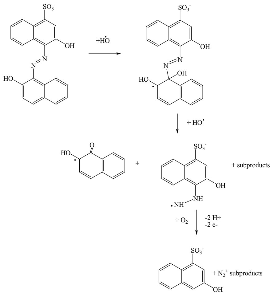
Fig. 8. A possible pathway of decomposition of Eriochrome Blue Black R to give \text{N}_2 .
